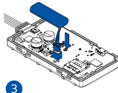
Figure 6 Battery connection
