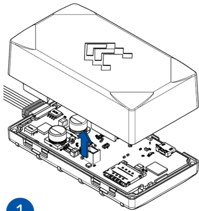
Figure 4 Cover removal
