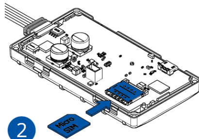
Figure 5 Micro SIM card insert
