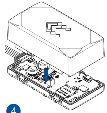
Figure 7 Attaching cover back
